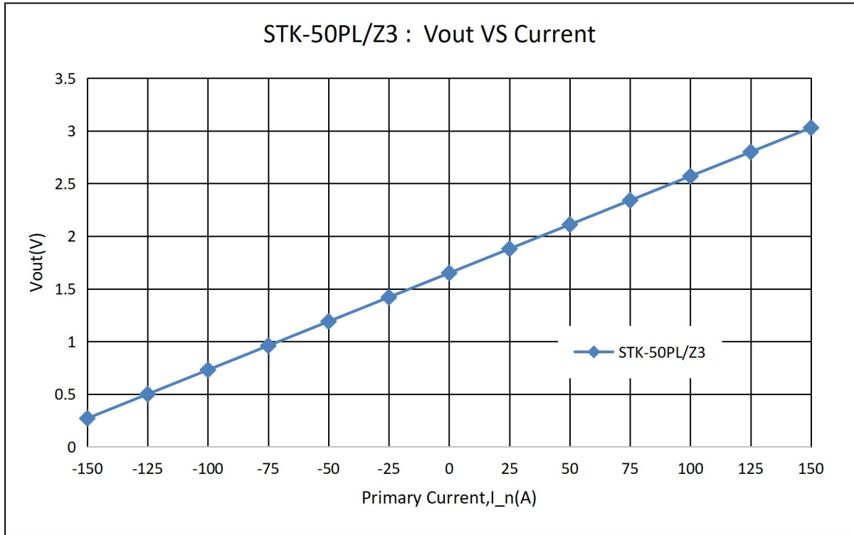
The dependence of Vout of STK-50PL/Z3 on the primary current.
