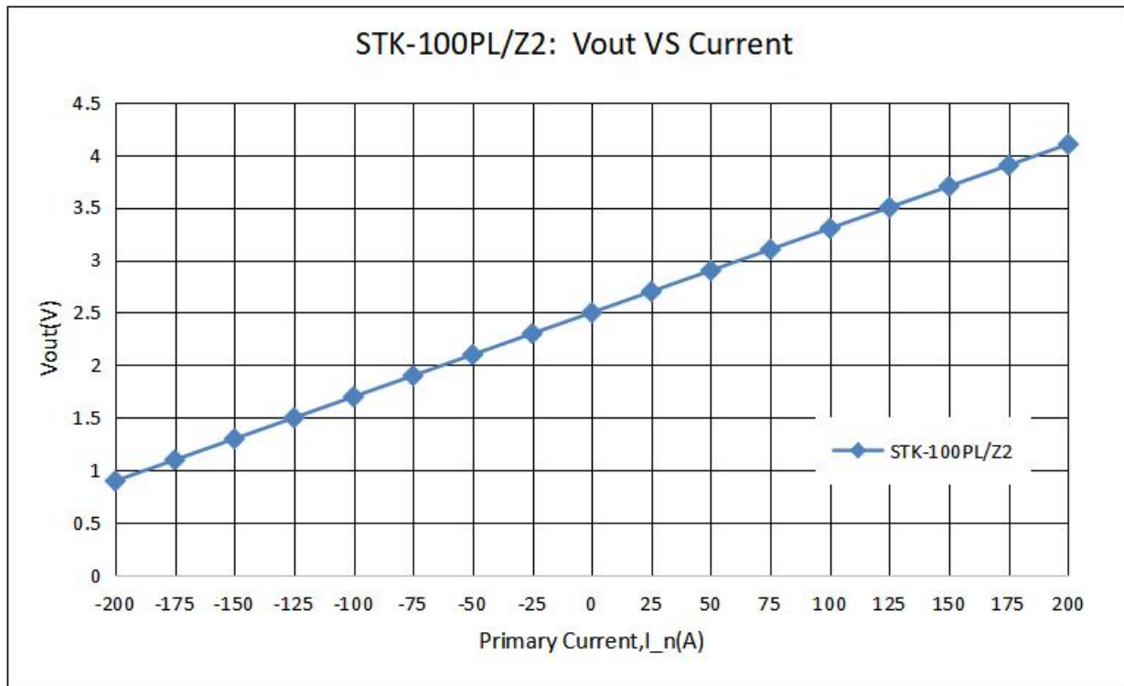
The dependence of Vout of STK-100PL/Z2 on the primary current.
